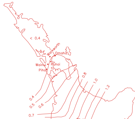
Figure 1 Seismic Zone Factor, Z , for Northland and Auckland from NZS 4297
